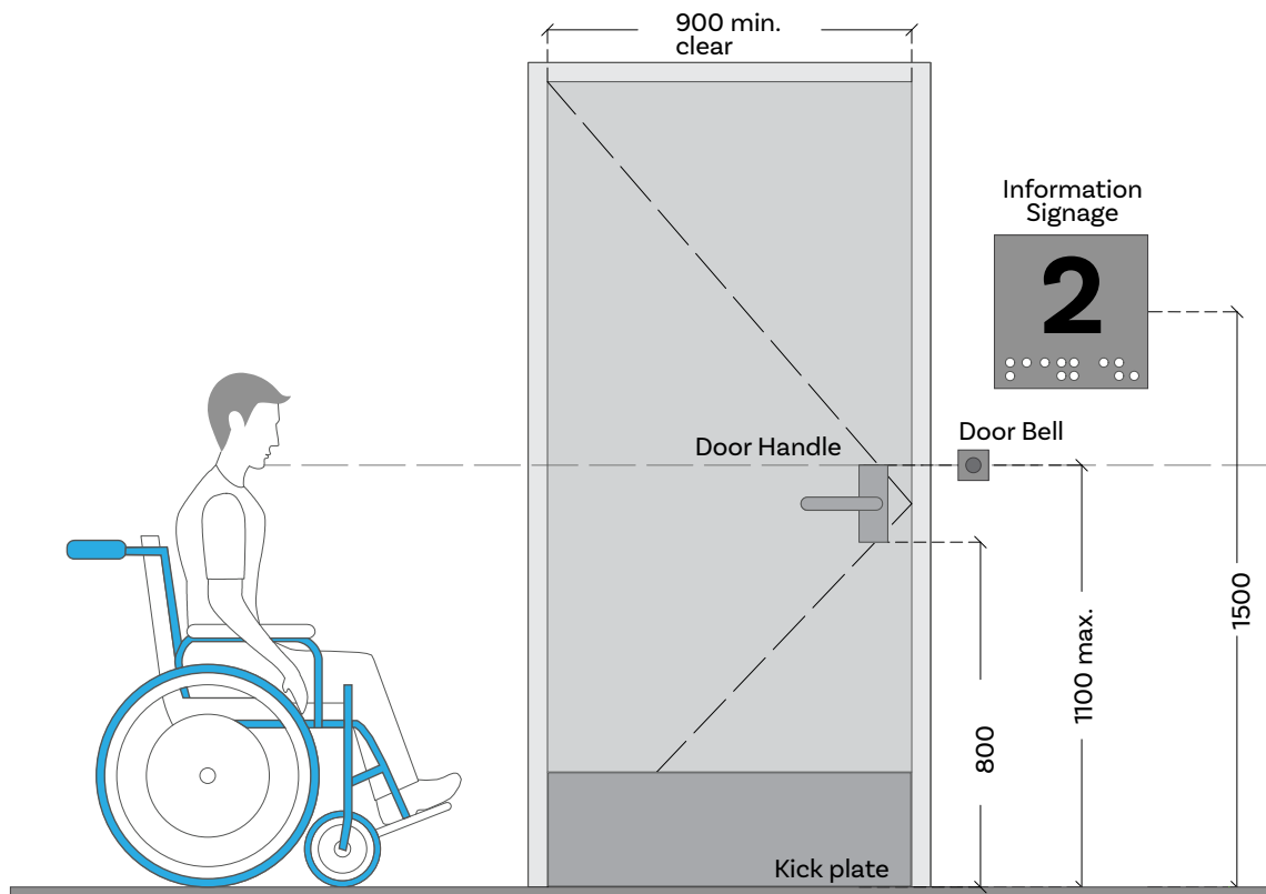
Figure 4.44 Door details
