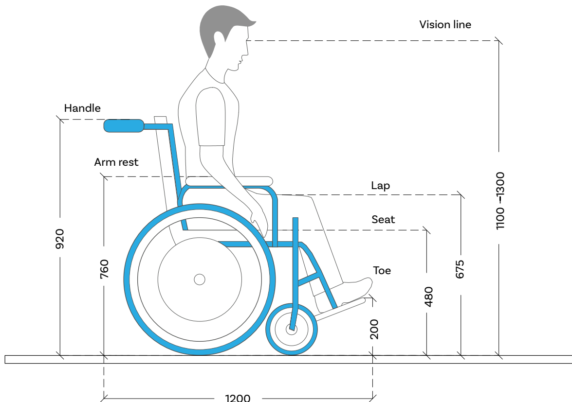
Figure 2.8 Wheelchair dimensions
