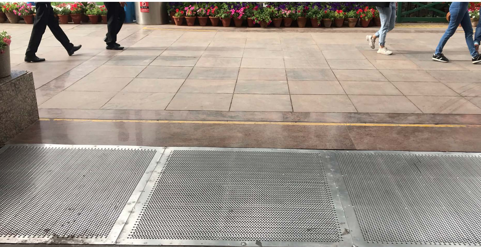
Image 3.12 Accessible grating details ( Perforated grating type) Photo Credits: Dr. Gaurav Raheja
