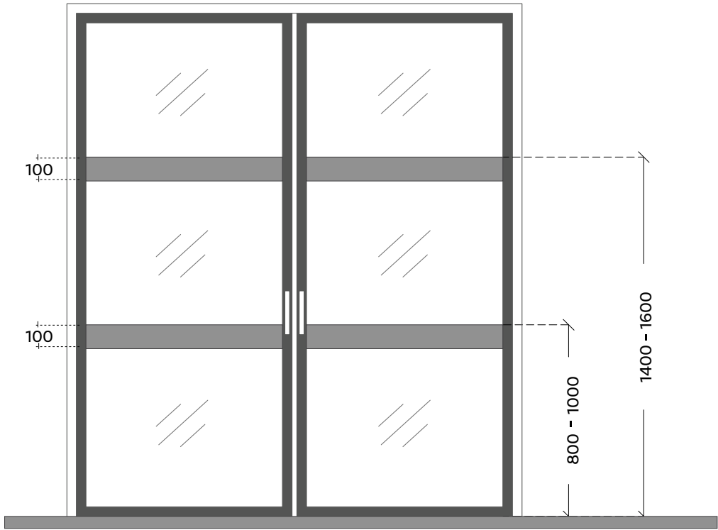
Fig b: Markings on Glass Doors
