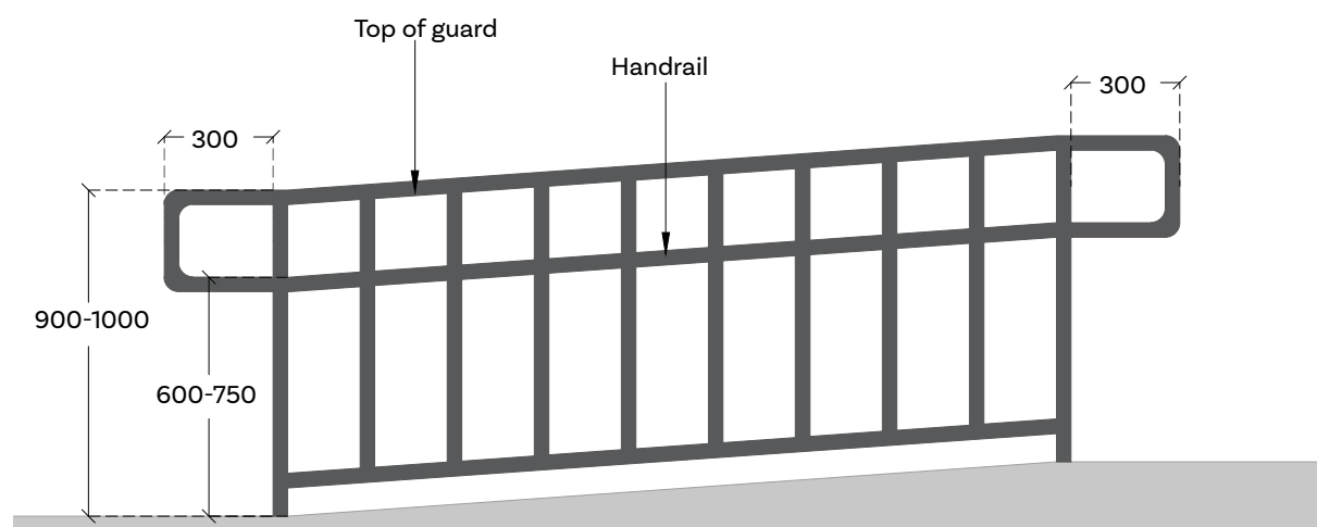
Figure 3.17 Handrail detail
