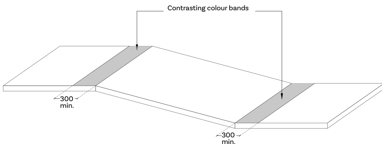
Fig b. Use of colour contrast or bands with colour contrast for rises from 15 to 200 mm
