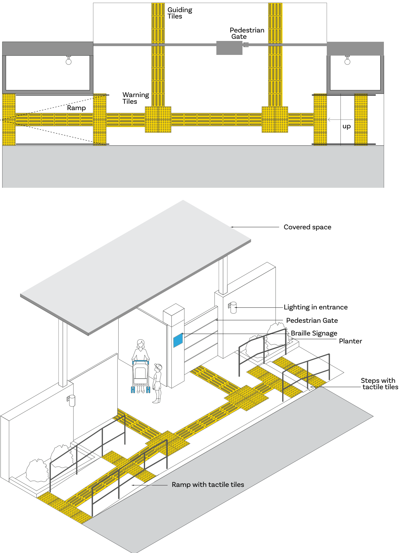
Figure 3.1 Accessible site entrances: Typical detail A
