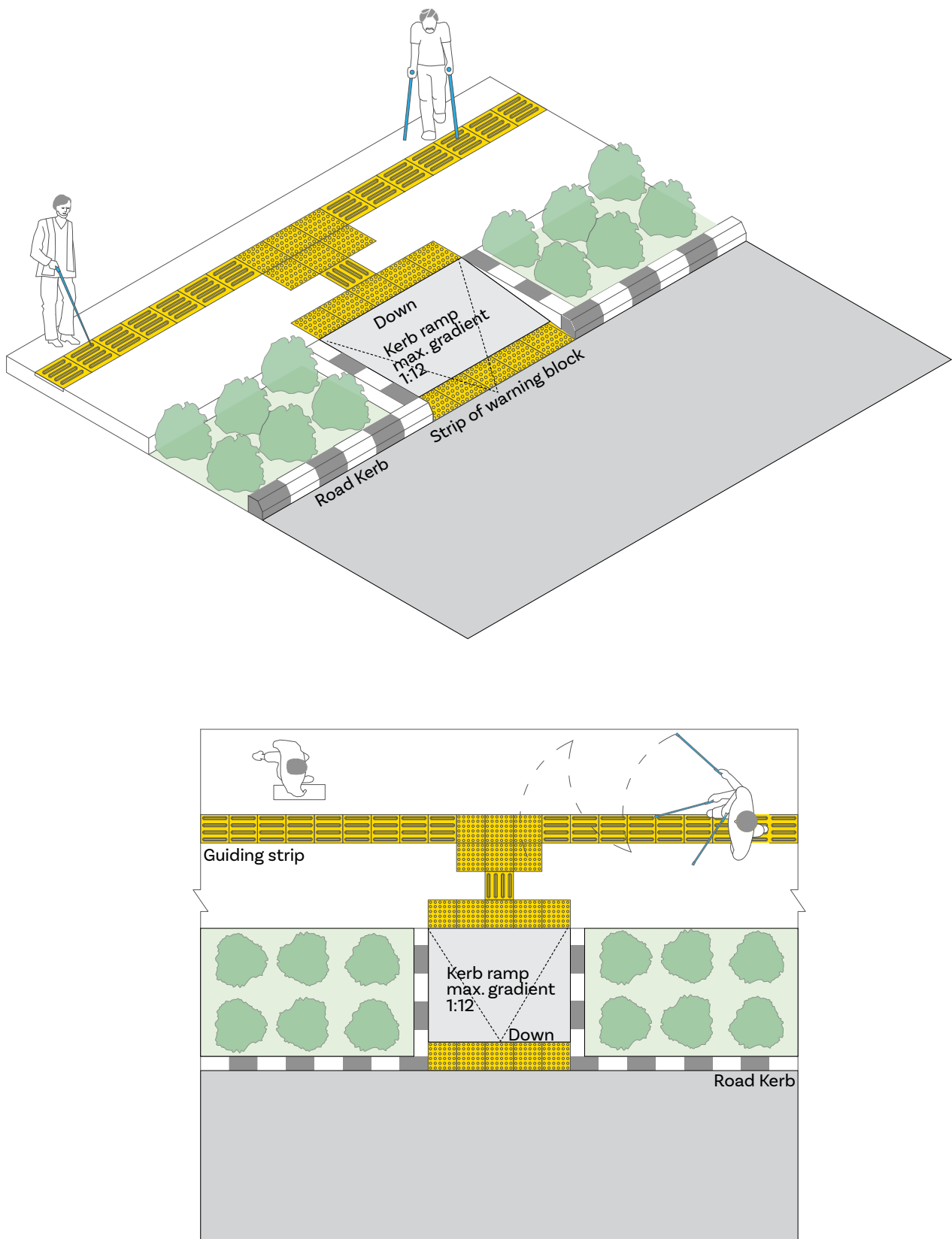
Figure 3.11 Accessible kerb ramp: Typical detail A
