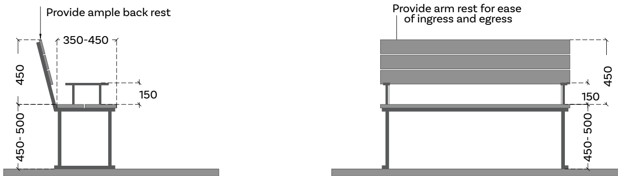
Figure 3.27 Outdoor seating: Elevation
