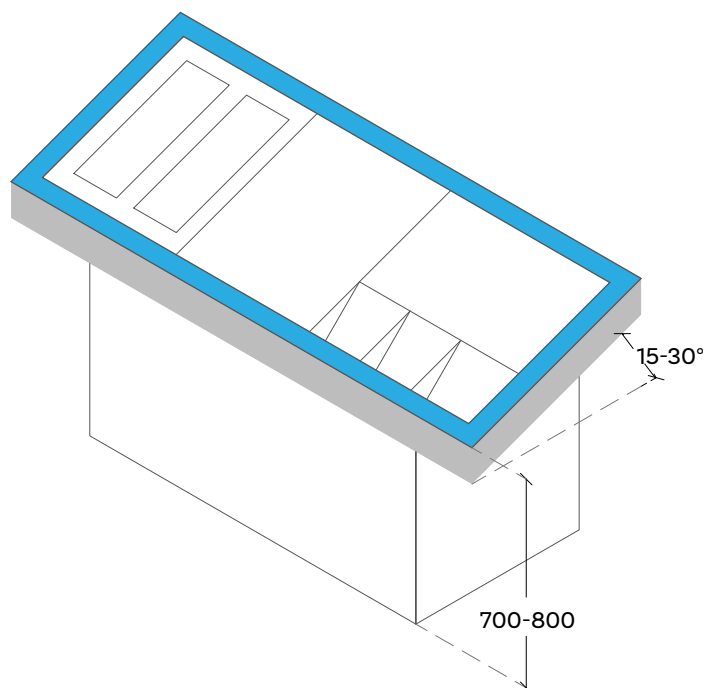
Figure 5.1 Information Display Counter
