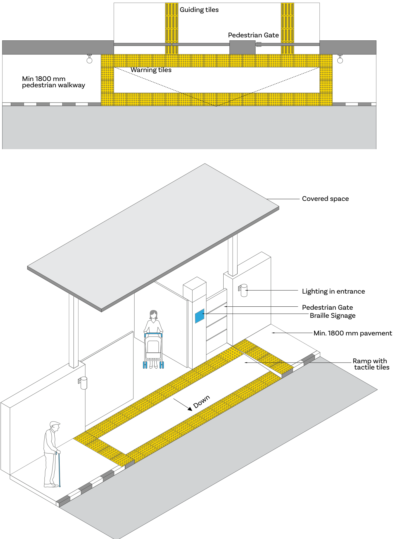
Figure 3.2 Accessible site entrances: Typical detail B
