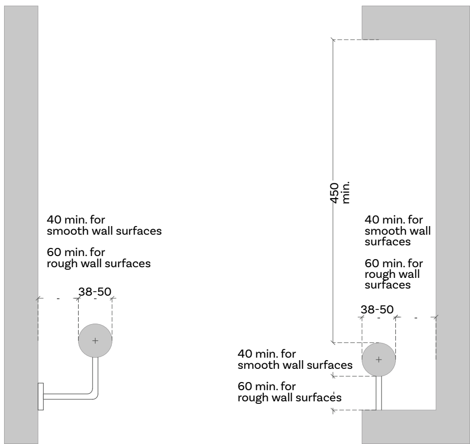
Fig b. Handrail clearance from the wall
