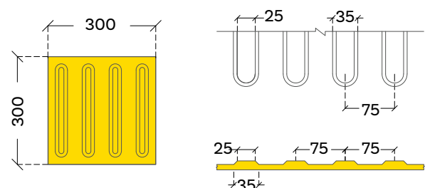
Fig b: Guiding Indicators
